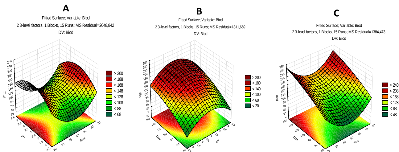
Fig. 2 Response surface plot and contour plot of the CAP biodegradation content as a function of (A) reaction time ( x_1 ) and pH of the medium ( x_2 ); (B) pH of the medium ( x_2 ) and CAP concentration ( x_3 ); (C) CAP concentration ( x_3 ) and contact time ( x_1 )
